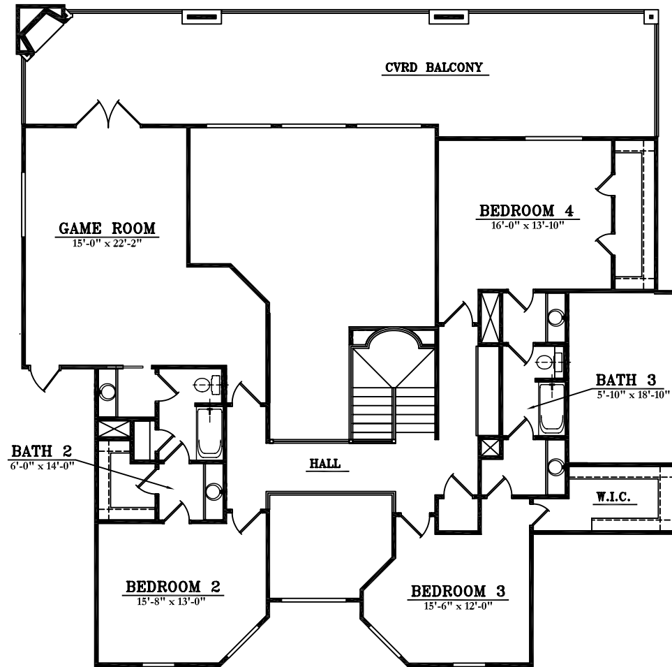
2nd floor
